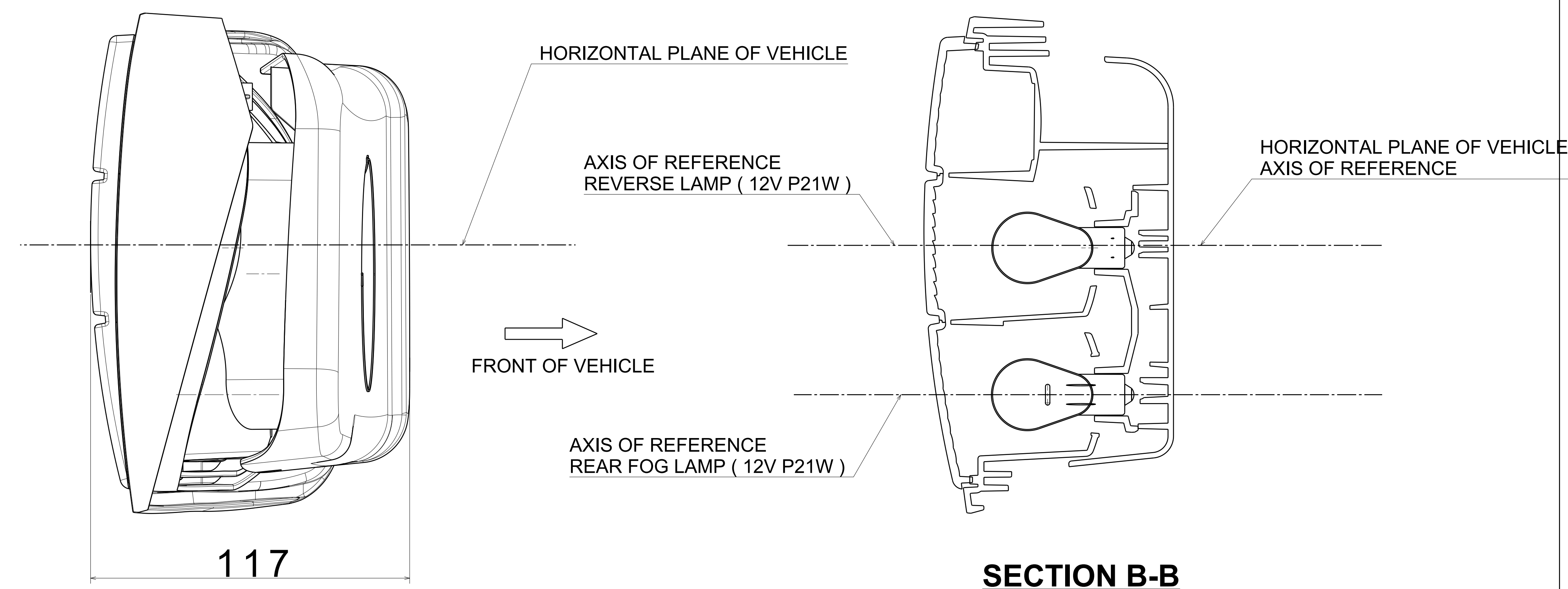
SIDE VIEW
